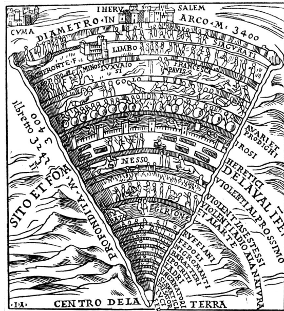
Figure 36: The nine circles of algebraic geometry.
