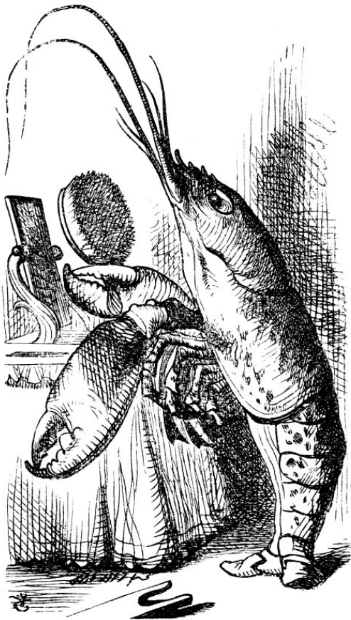
Figure 4: A student new to topology struggling to understand the hairy ball theorem.
